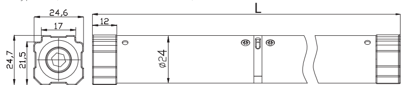
type VB (6mm hex - for venetian blinds)
