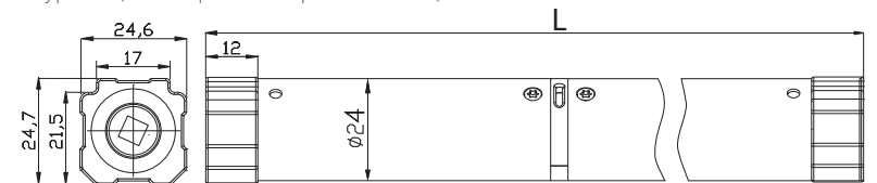
type PB (5mm square - for pleated blinds)
