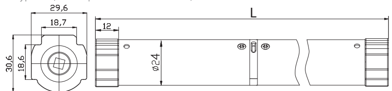
type RS (5mm square - for roman blinds)
